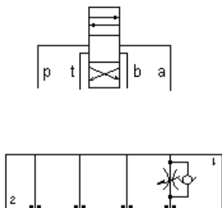
Flow Control, Meter-In A
