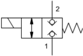
X-Control, C-Poppet
